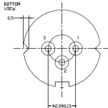
Pin Configuration
