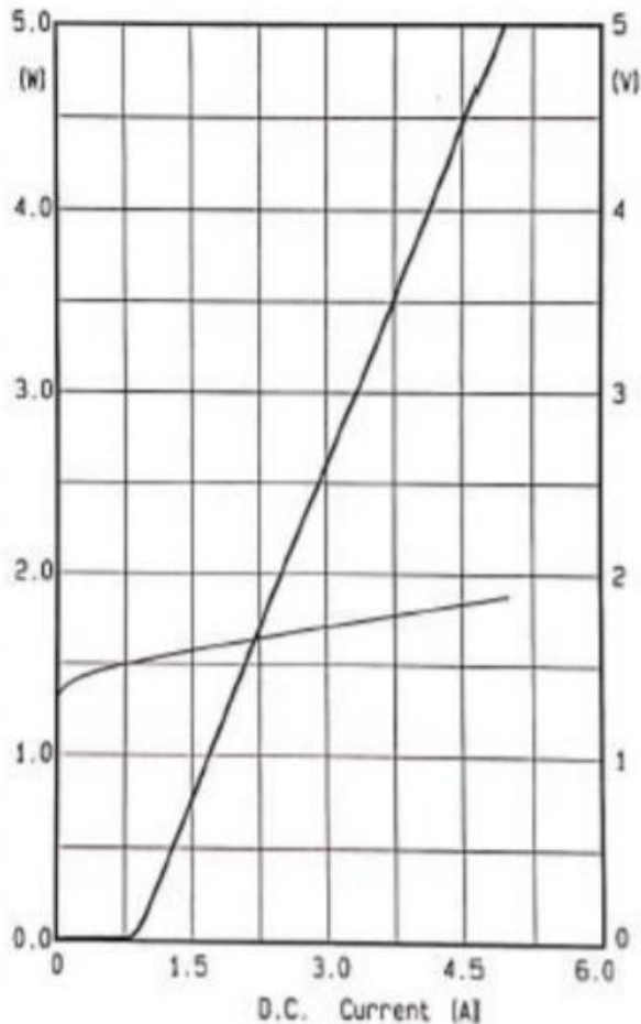
P-I-V Curve
