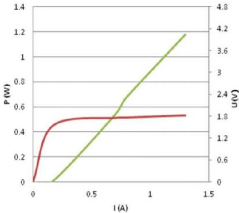
P-I-V Curve
