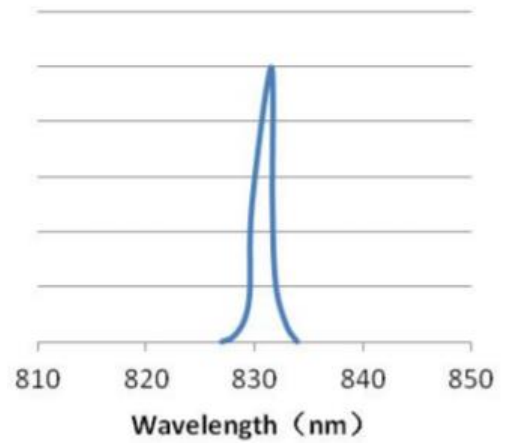
Spectral Curve
