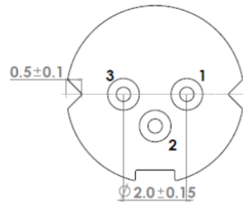
Pin Configuration
