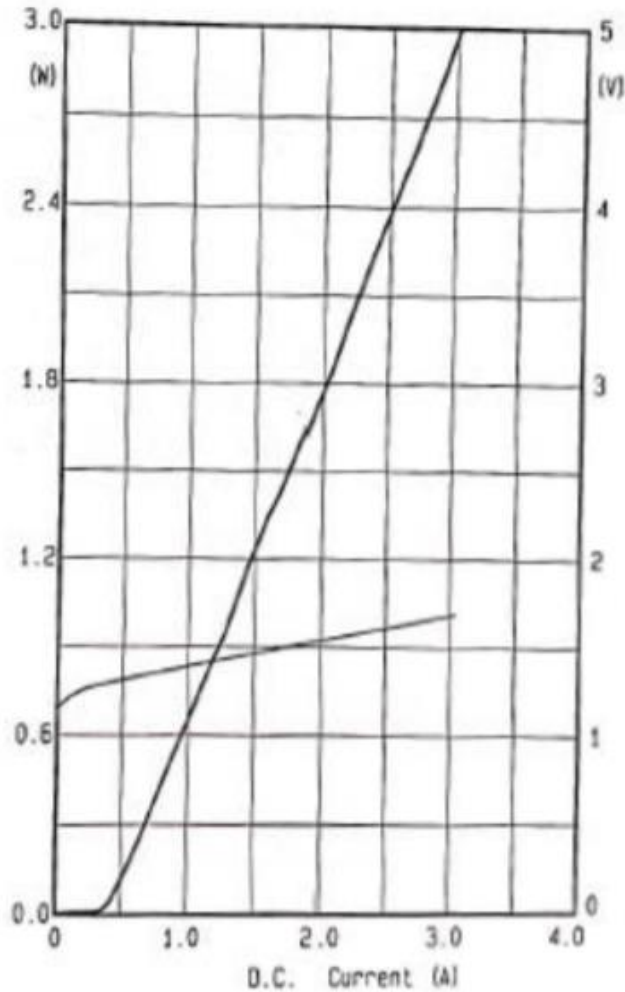
P-I-V Curve
