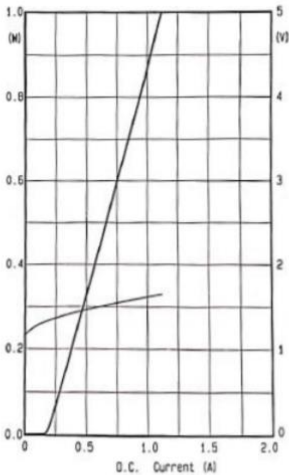
P-I-V Curve
