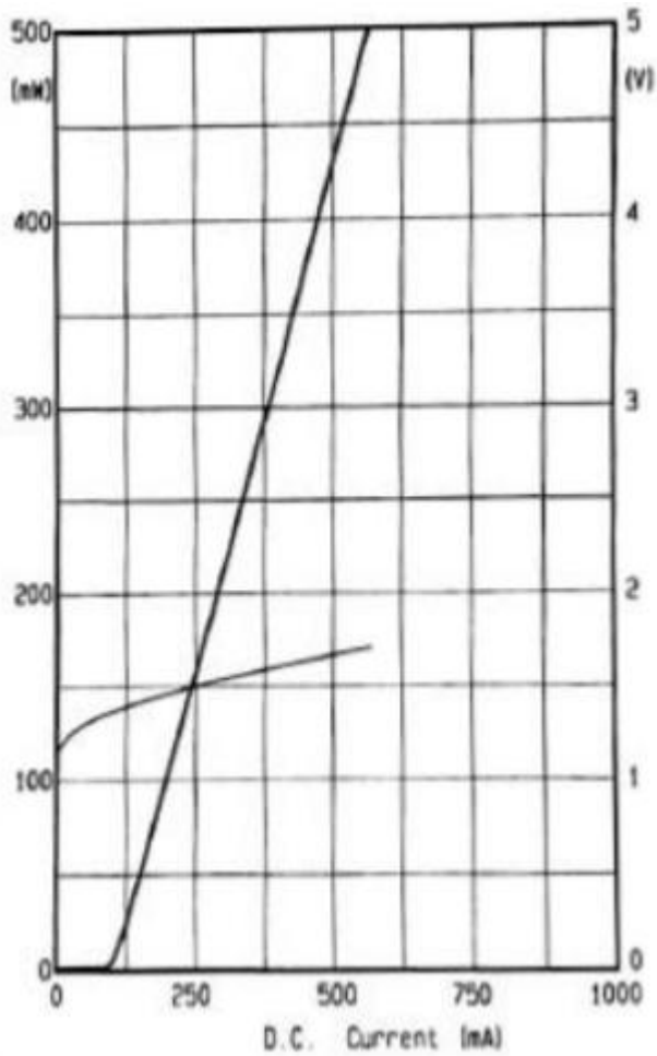
P-I-V Curve
