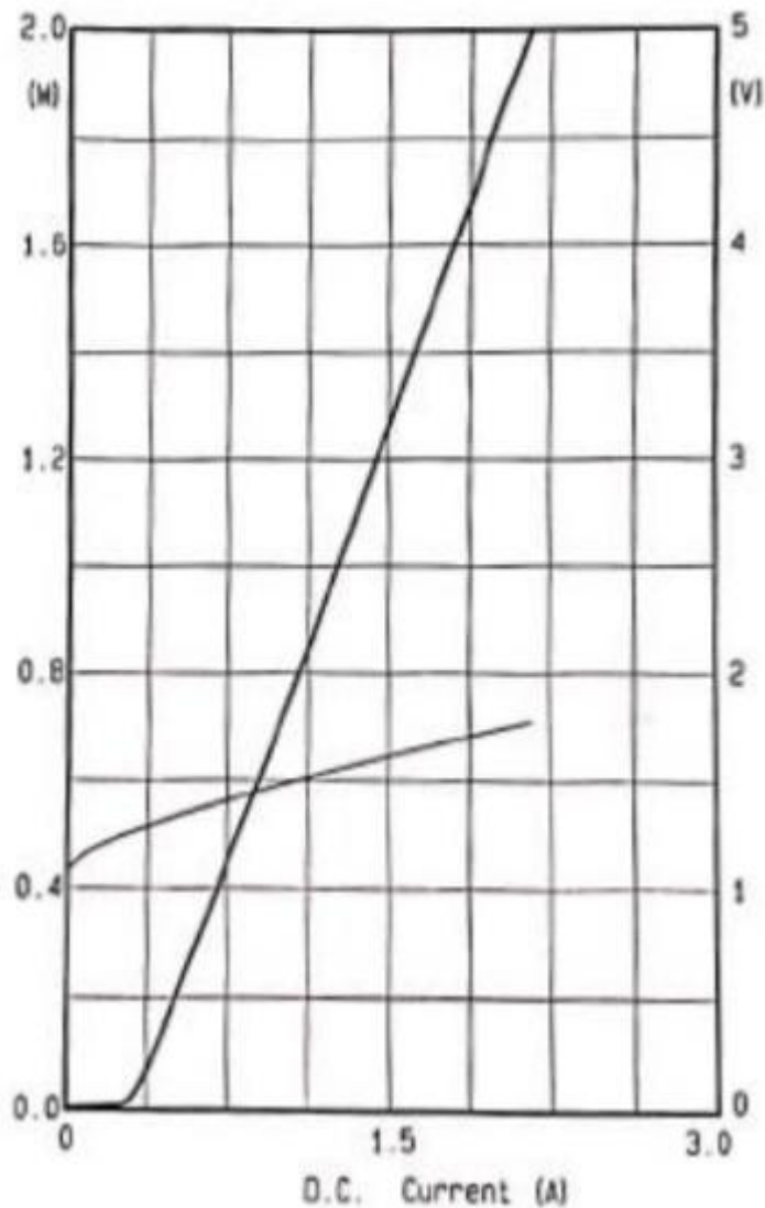
P-I-V Curve
