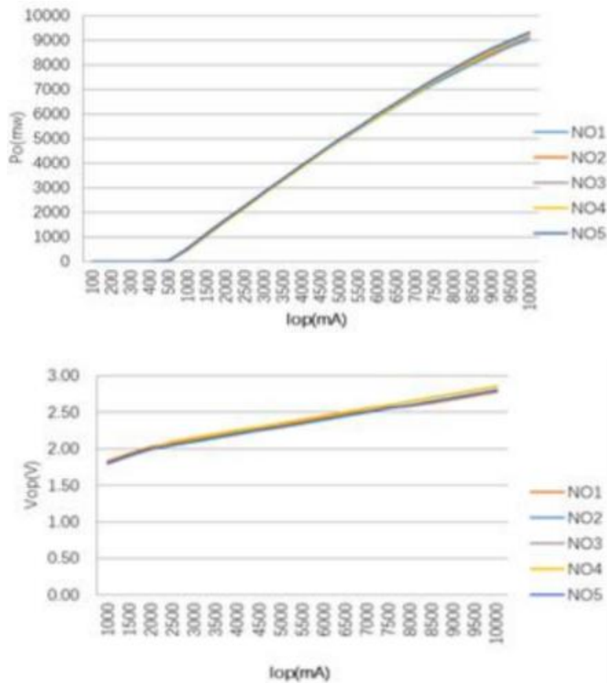
P-I-V Curve
